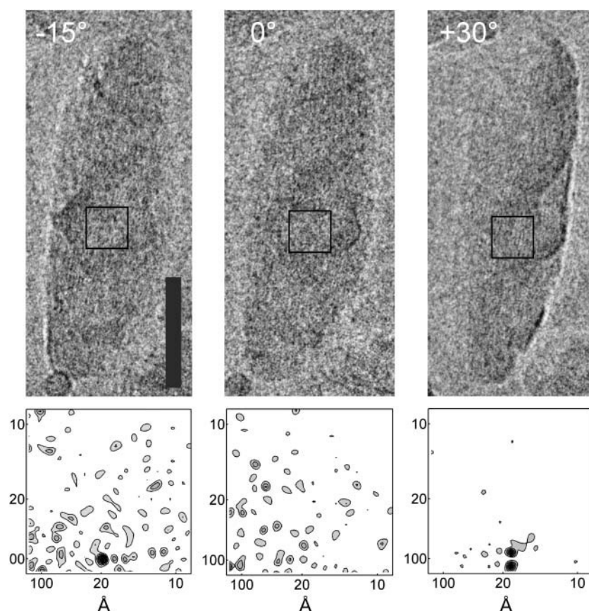
FIGURE 2 (Upper panels) Tilted series images ( -15^\circ , 0^\circ , and 30^\circ ) of a representative chlorosome. Bar, 500 Å. The defocus value was 1.6\ \mu\text{m} . The tilt axis is oriented almost parallel to the striae and intersects through the middle of the chlorosome. Lower panels show the power spectra computed from the boxed regions (shown as a square in each upper panel), which were selected to correspond to the same volume of the chlorosome throughout the tilt.
